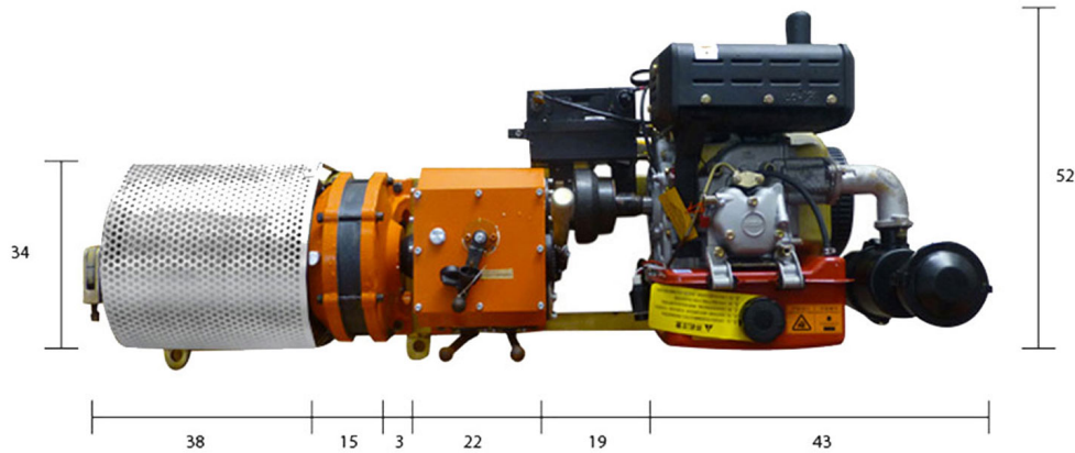
Dimensions in cms / Dimensiones en cms
